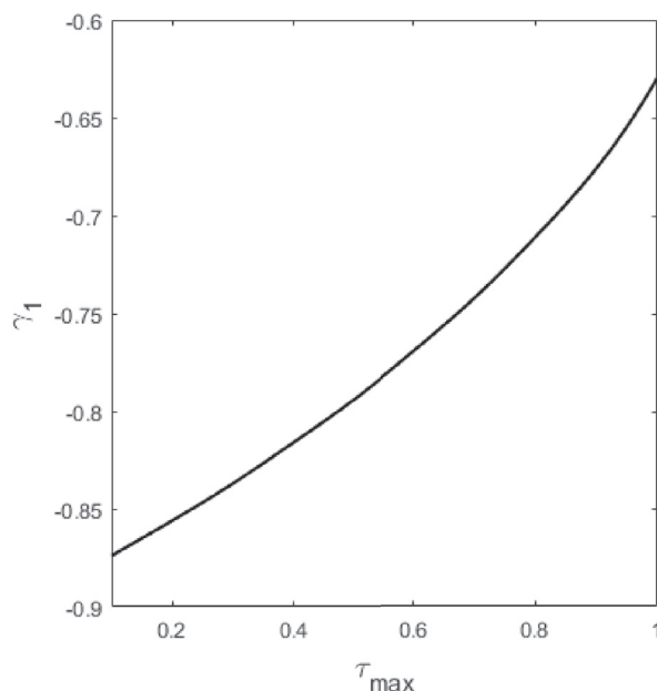
Fig. D1 The relationship between \gamma_1 and \tau_{\max} .
